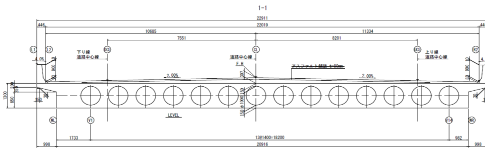
(A1~P1間)
